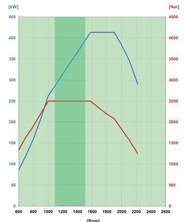
CURSOR 13 - 560HP E4/E5
